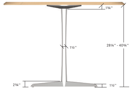
Elevation View of Vue Base
