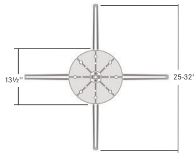
Plan View of Vue Base
