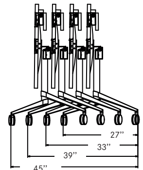
Nesting Configuration: Side view of four tables nested. Approximate dimensions.
