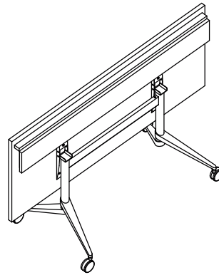
Folding table with modesty panel with 9" grommet and YEC electrical module
