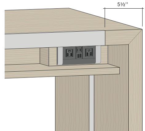
Miter corner with aluminum trim. Specify edge style AL.
