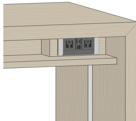
Miter corner with wood trim. Specify edge style WD.
