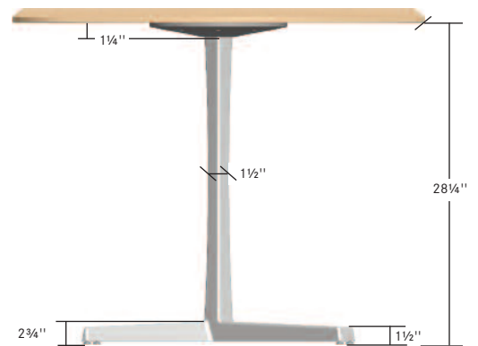
Elevation View of Revue Base
