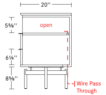
Section View
