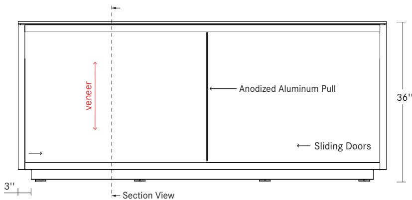
Front View/Serving Height
