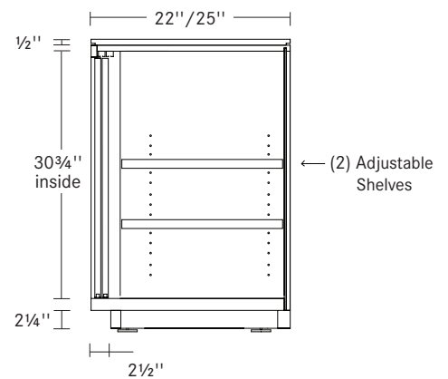
Section View/Serving Height
