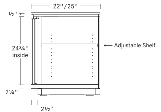
Section View/Standard Height
