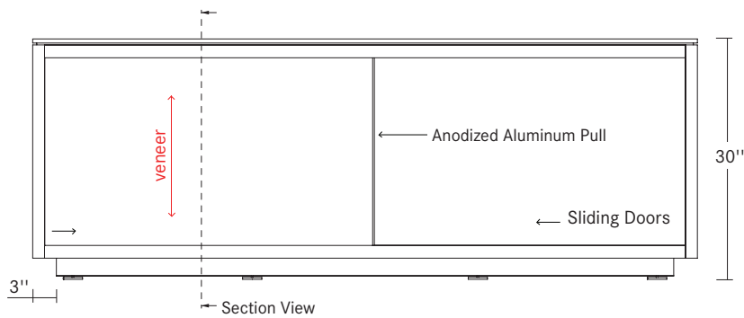
Front View/Standard Height
